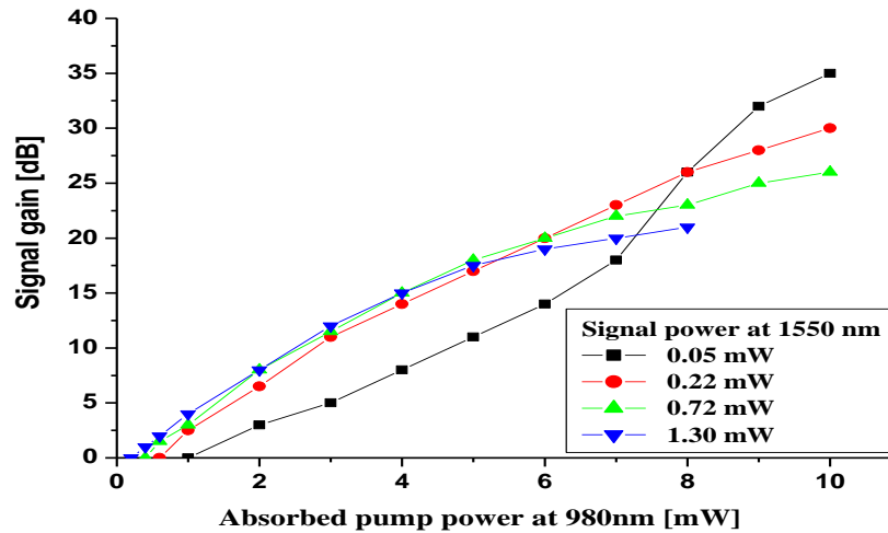
Figure 5: Signal gain (in dB) at 1550 nm as a function of absorbed power at 980nm
