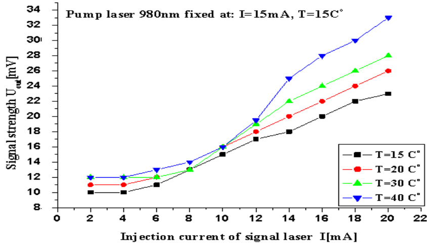
Figure 4: Signal strength in mV versus the injection current in mA of signal laser 1550 nm by fixed I= 15 mA at T=15 C° of pump laser 980nm
