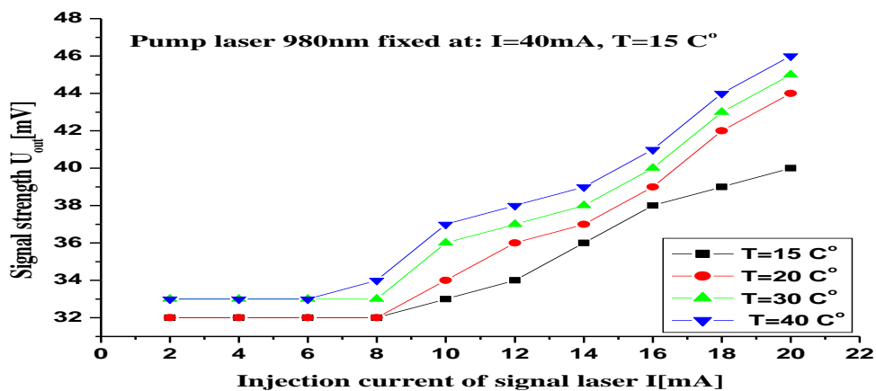
Figure 2: Signal strength in mV versus the injection current in mA of signal laser 1550 nm by fixed I= 40 mA and T=15 C° of pump laser 980nm
