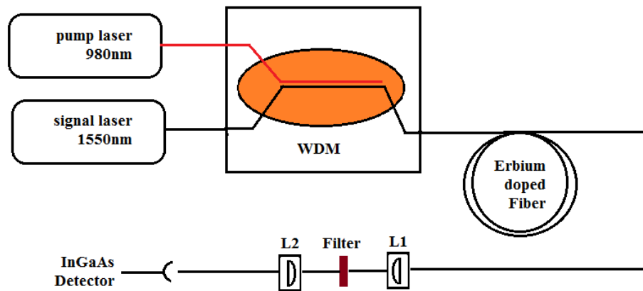
Figure 1: Schematic diagram of the EDF experiment
