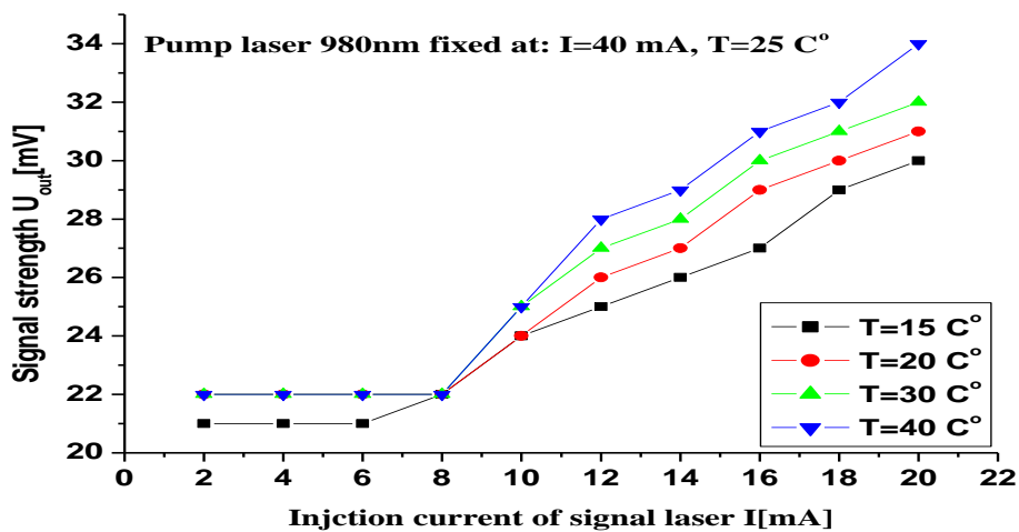
Figure 3: Signal strength in mV versus the injection current in mA of signal laser 1550 nm by fixed I= 40 mA and T=25 C° of pump laser 980nm
